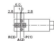
YSV10-DP-M-*** Normally Open Type
