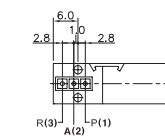
YSV10-DP-L-*** Normally Closed Type
