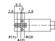
YSV10-DP-M-*** Normally Closed Type
