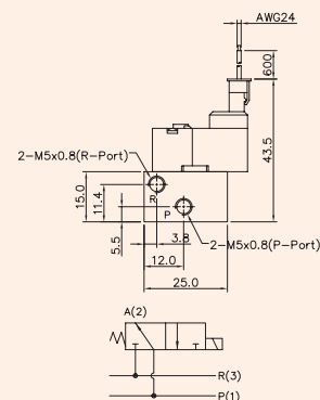
Normally Open Type
