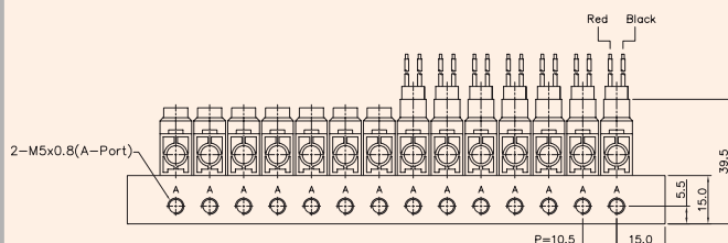
3-PORT MANIFOLD BLOCK DIMENSION
