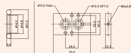
Single Acting Use Plate SN3000-Plate
