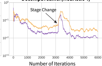
DecompDreamer(Heuristic 4)
