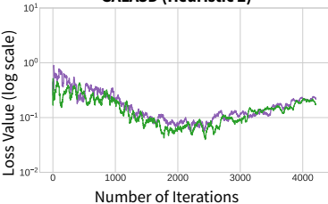
GALA3D (Heuristic 2)
