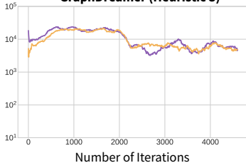
GraphDreamer (Heuristic 3)
