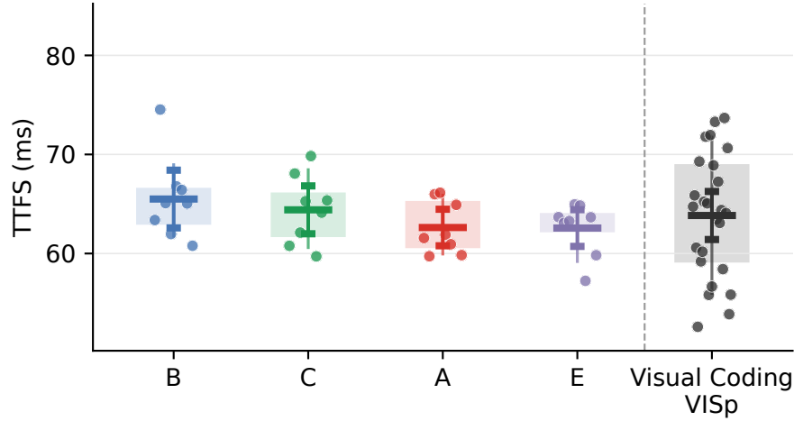
V1: within-area locations + Visual Coding VISp
