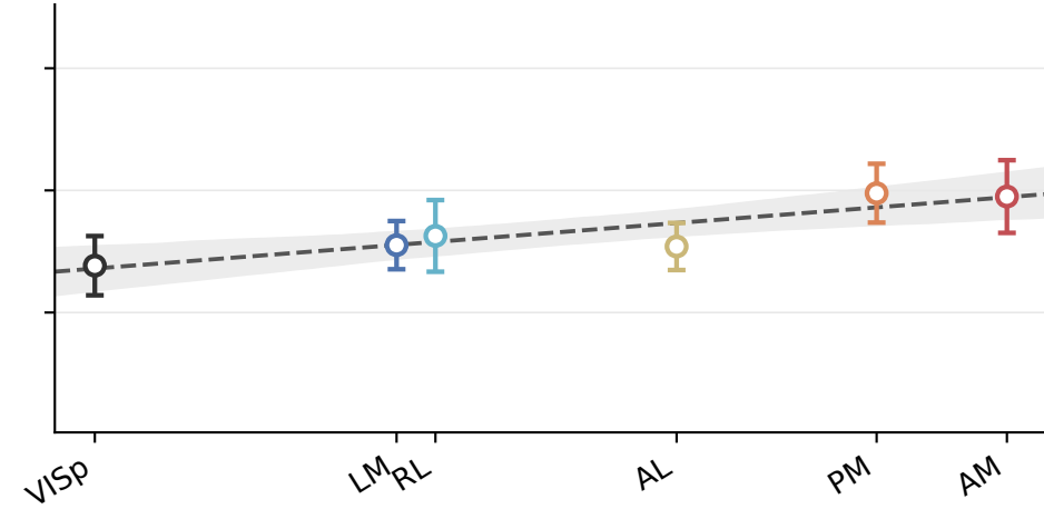
Visual Coding areas by hierarchy score
