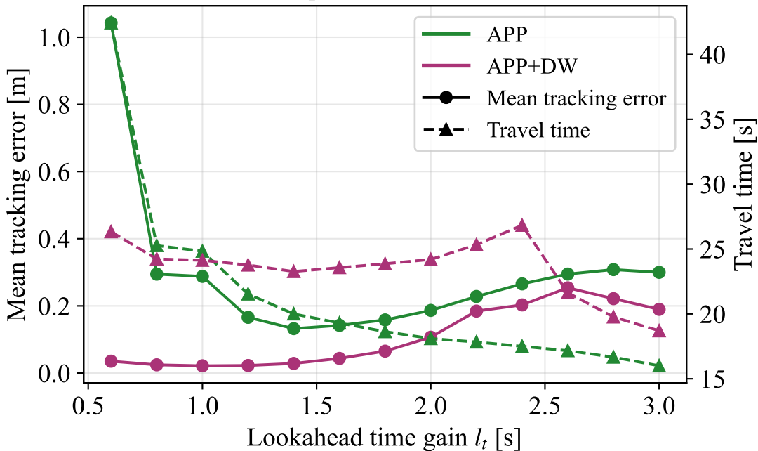
PathC: adaptive-lookahead trade-off
