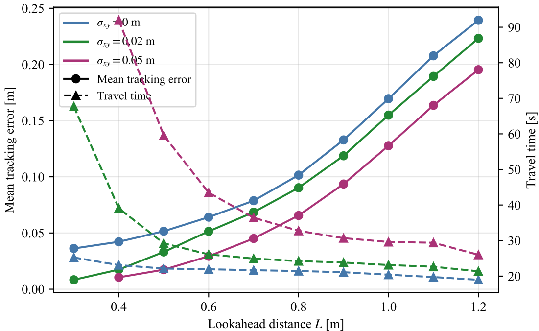
PathC: fixed-lookahead trade-off
