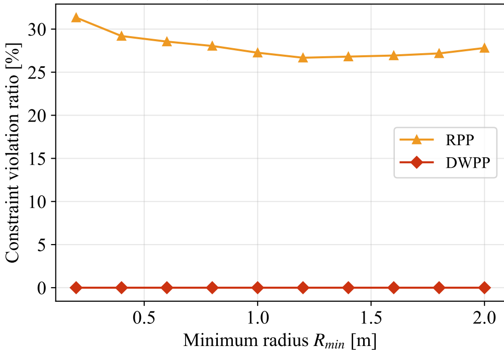
PathC: dynamic-constraint violations
