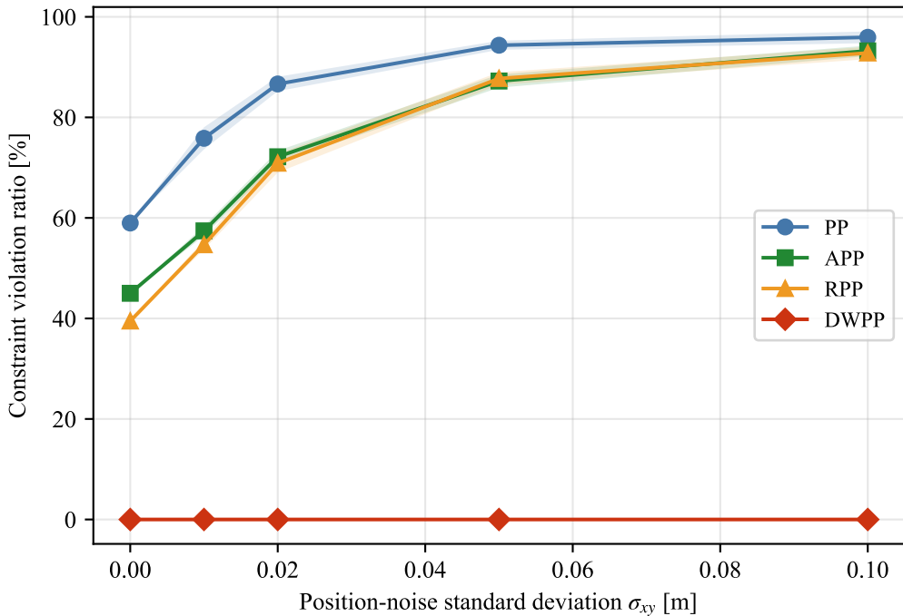
PathC: violations under localization noise
