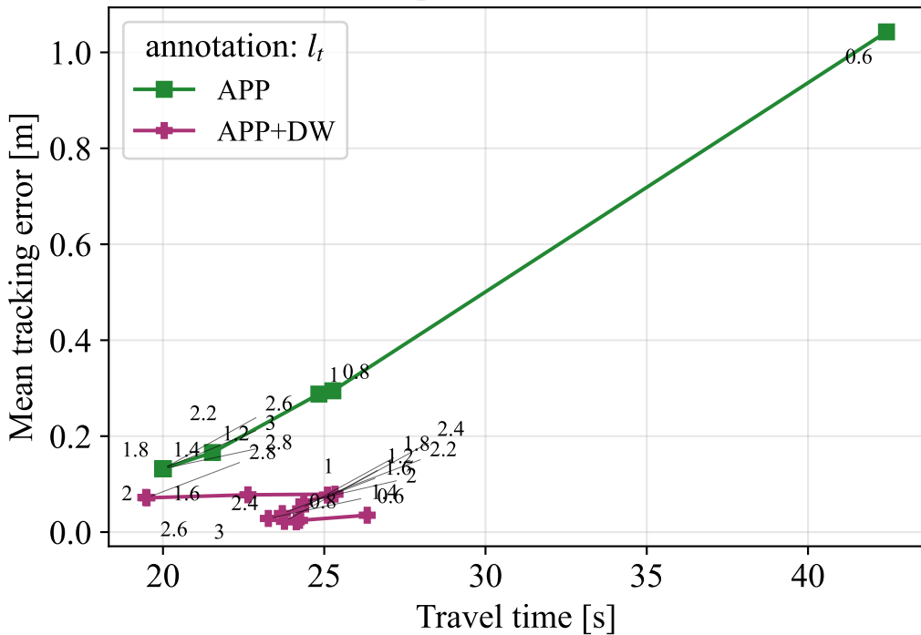
PathC: adaptive-lookahead trade-off
