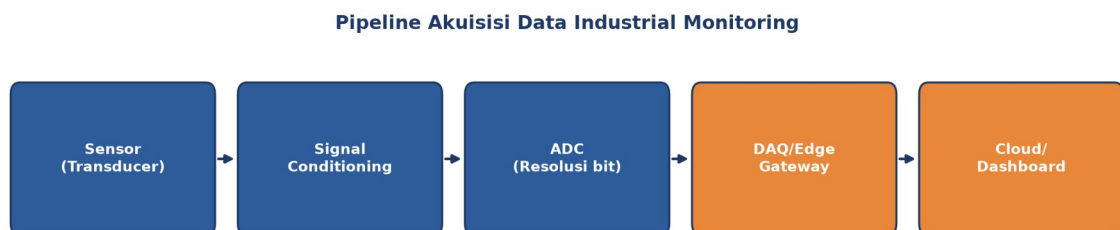
Gambar 6. Pipeline akuisisi data industrial monitoring: sensor, signal conditioning, ADC, DAQ/edge gateway, hingga cloud/dashboard.
