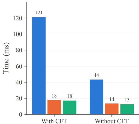
Witness
