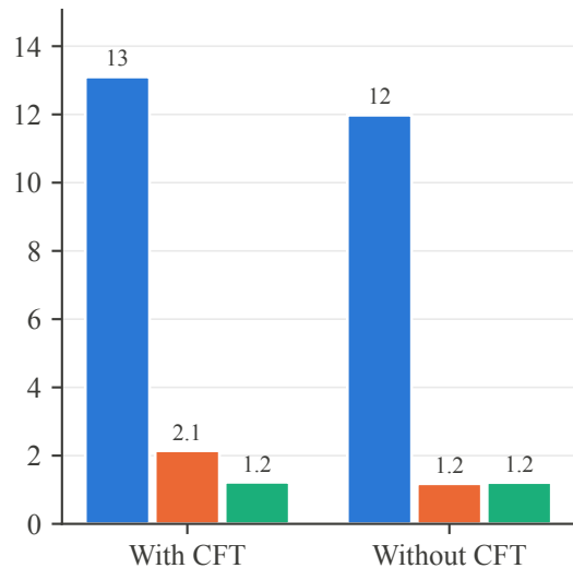
Verify
