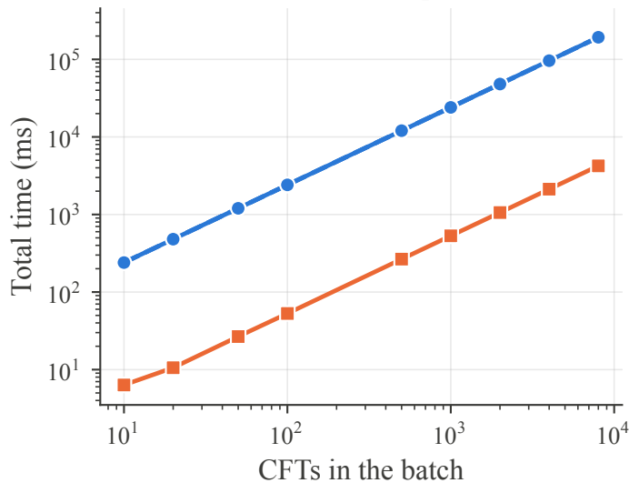
Direct decrypt
