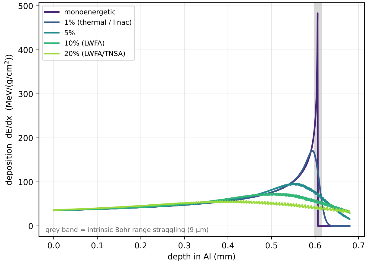
10 MeV protons: source energy spread washes out the Bragg peak
