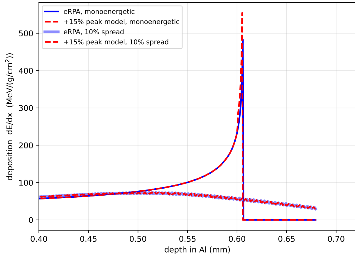
A 15% stopping-model difference vanishes at 10% energy spread
