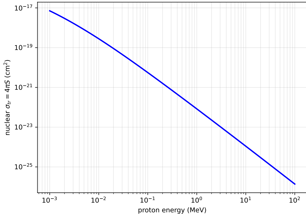
Nuclear transport cross section (same integral as nuclear stopping)
