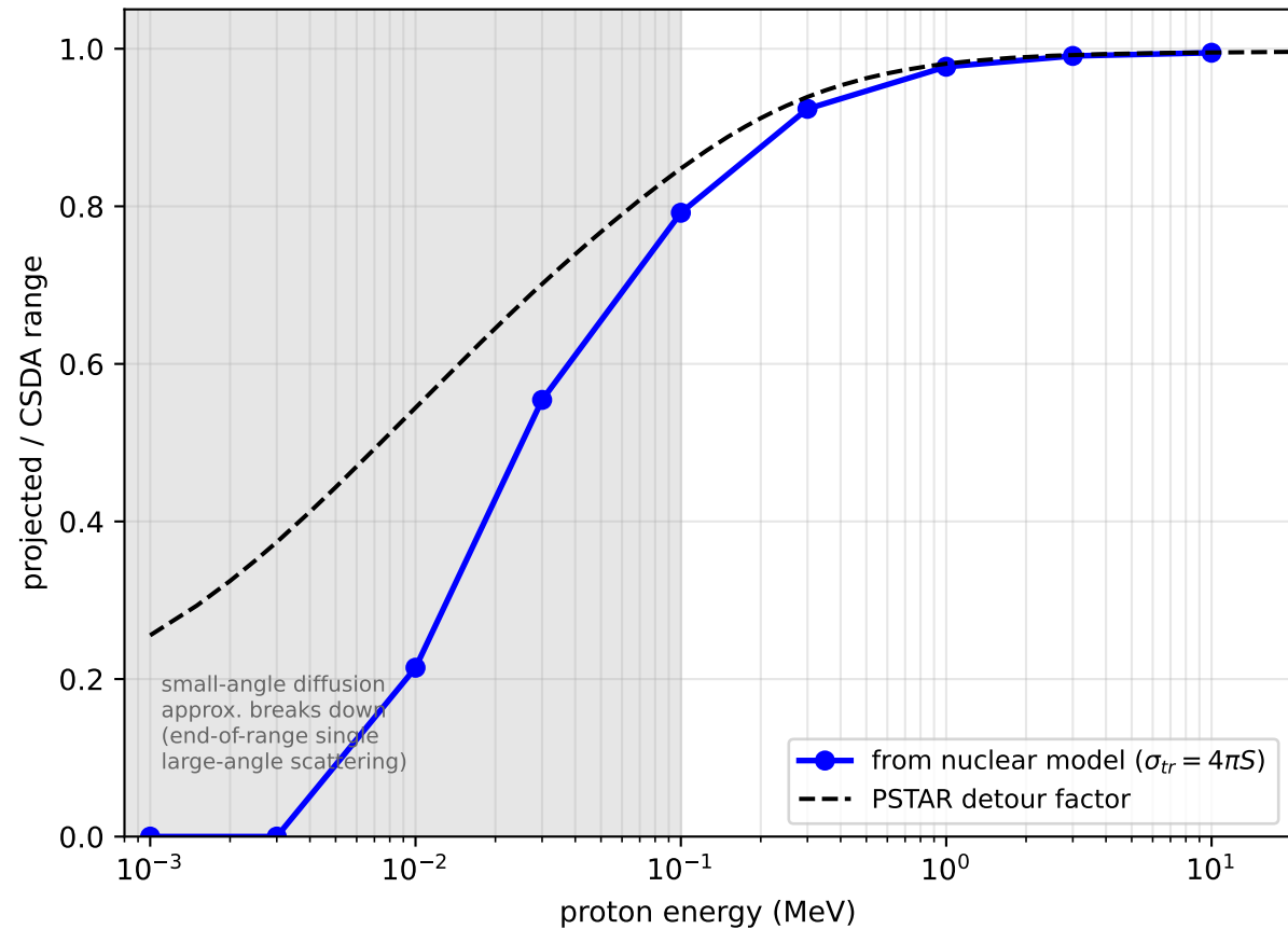
Pathlength-to-projected-range detour: model vs PSTAR
