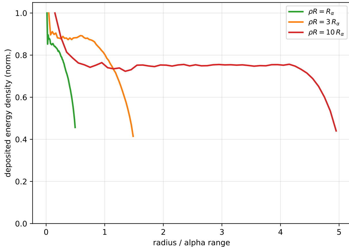
Hot-spot alpha deposition is volumetric — no Bragg peak
