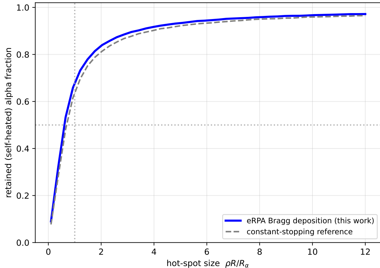
Self-heating is set by the integrated range, not the Bragg shape
