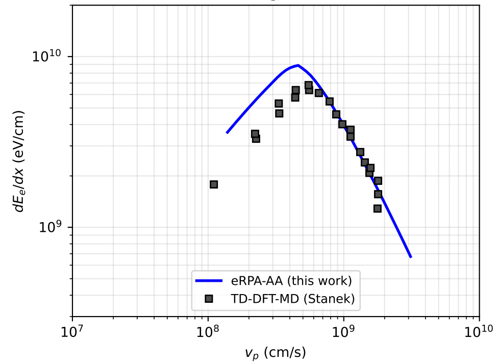
(a) H, 1 g/cc, 2 eV
