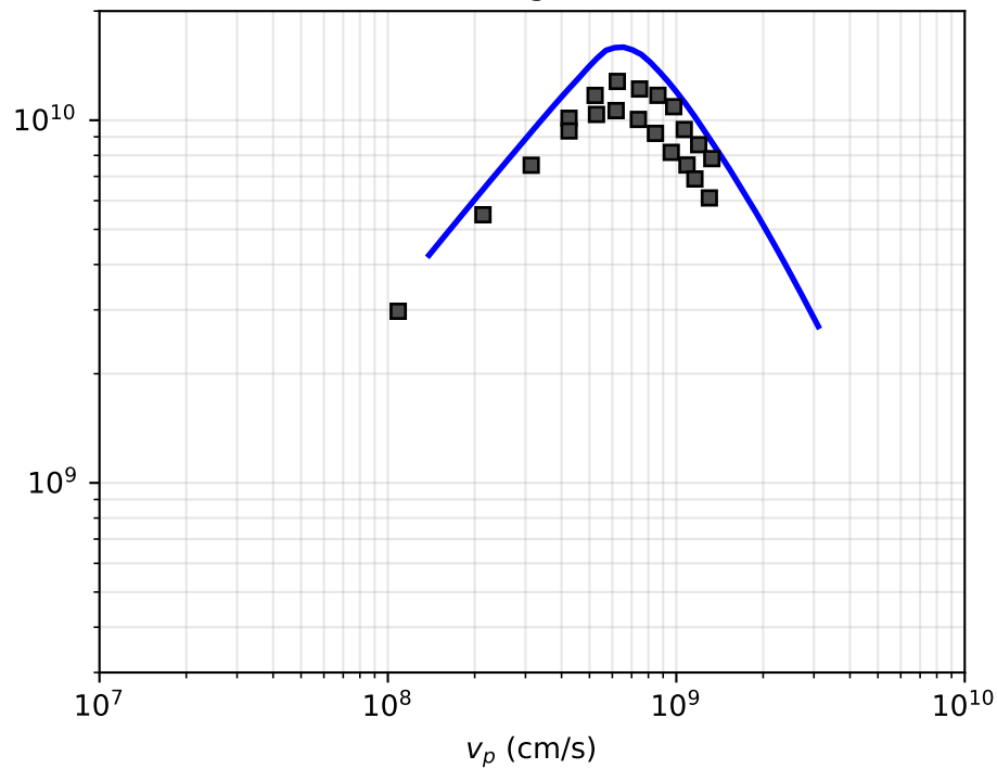
(b) C, 10 g/cc, 2 eV
