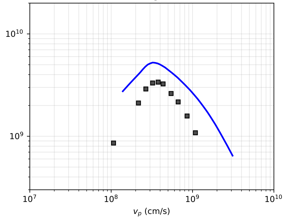
(c) Al, 2.7 g/cc, 1 eV
