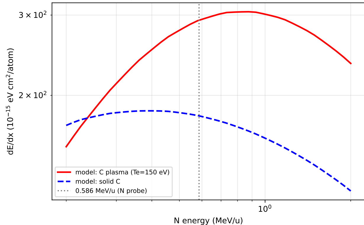
Cayzac 2017: N ions in carbon plasma
