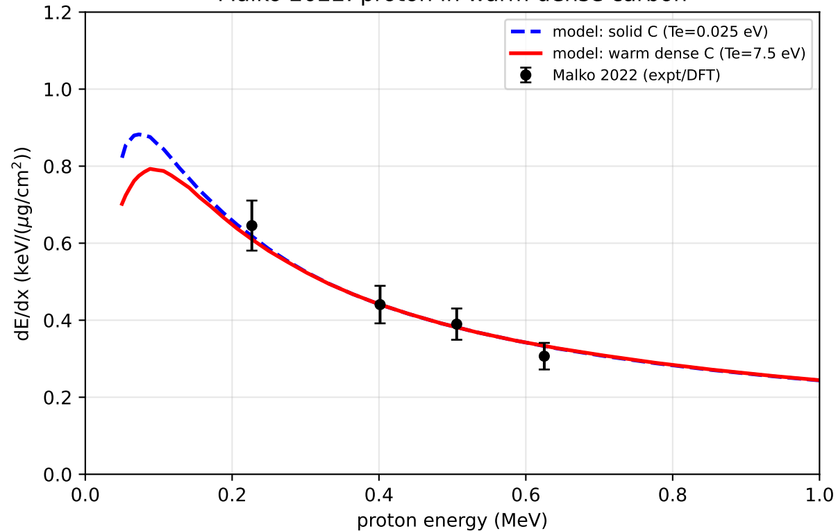
Malko 2022: proton in warm dense carbon
