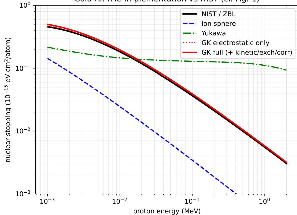
Cold Al: FAC implementation vs NIST (cf. Fig. 1)
