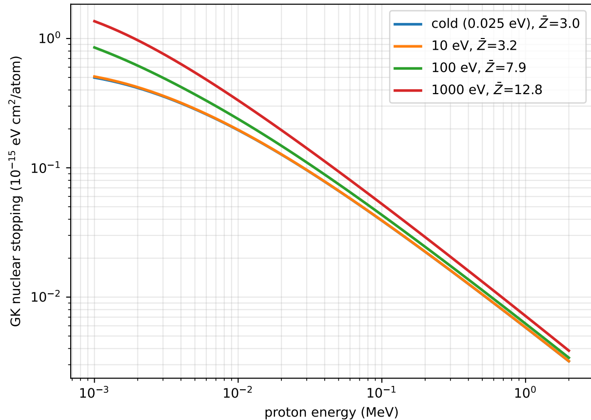
Al: nuclear growth with Te (FAC Zbar; cf. Fig. 2)
