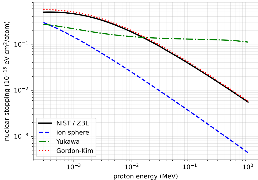
Proton in cold solid-density Al (cf. Faussurier Fig. 1)
