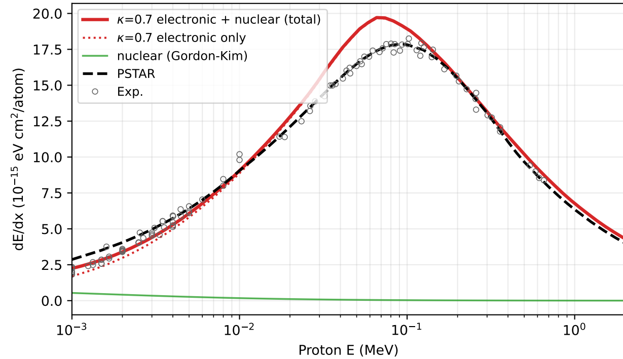
H2O ( E_g \sim 7 eV)
