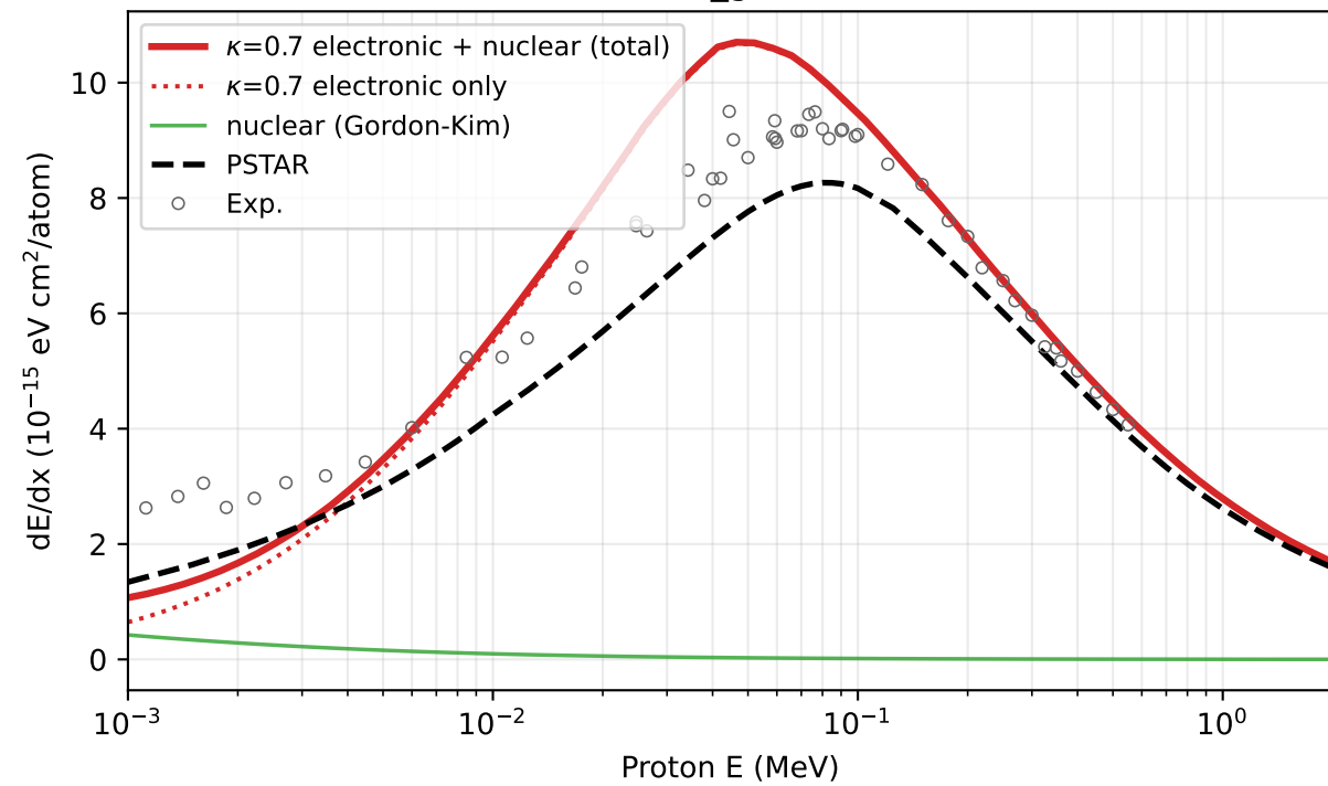
H2O ( E_g \sim 7 eV)
