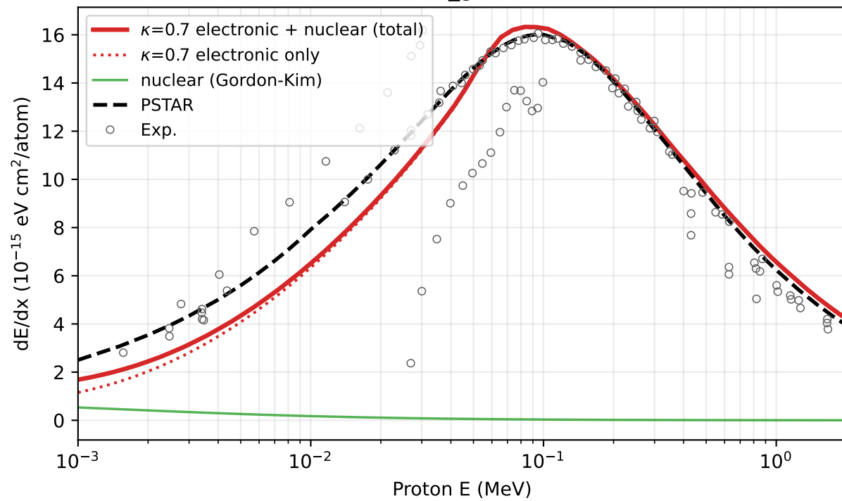
Al2O3 ( E_g \sim 8.8 eV)
