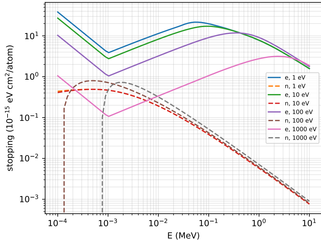
Proton in Al: electronic (solid) + nuclear/GK (dashed)
