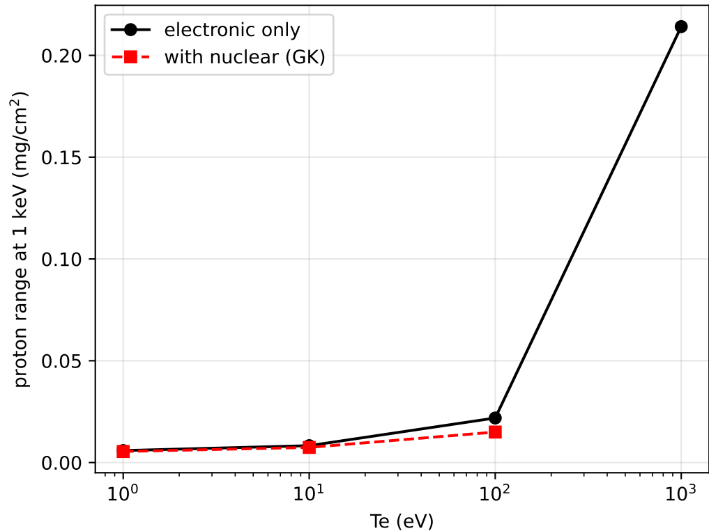
Range reduction from nuclear stopping (cf. Fig. 3)
