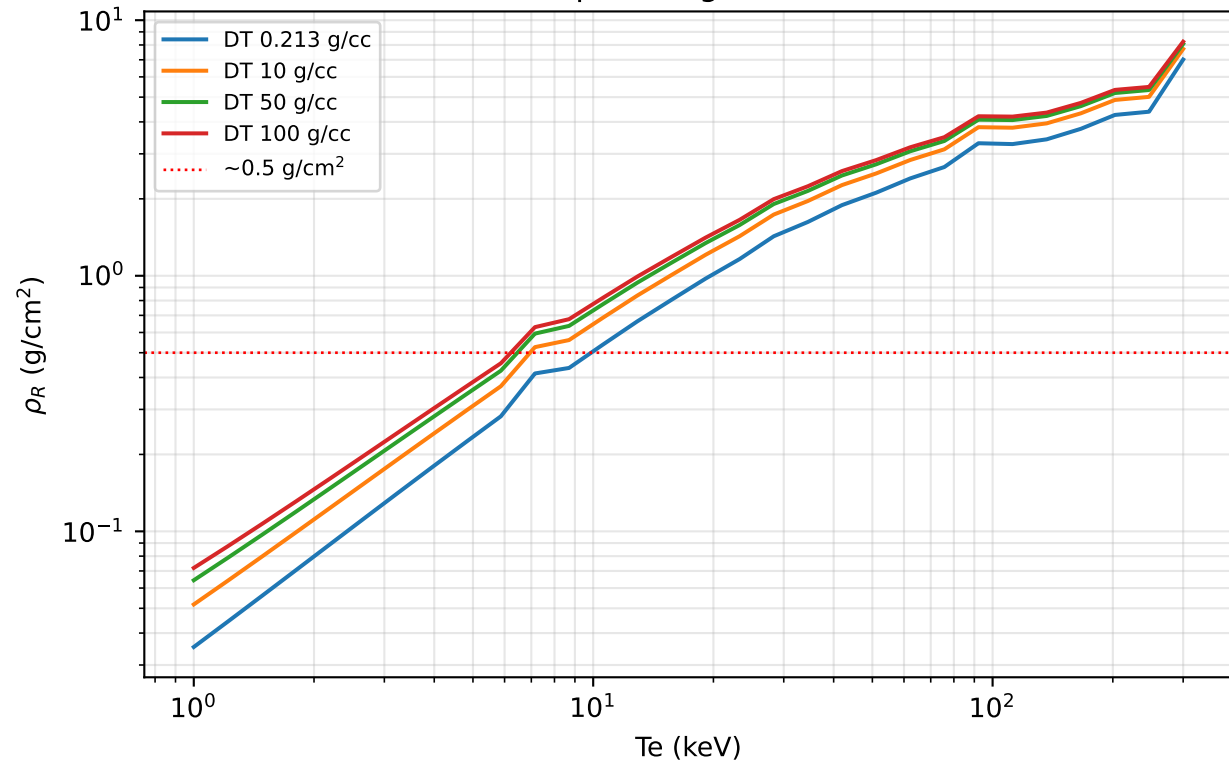
Alpha range in DT
