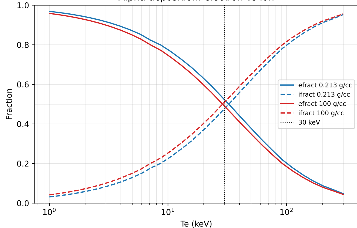
Alpha deposition: electron vs ion
