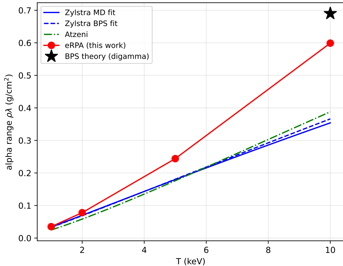
DT 10 g/cc: alpha range vs T
