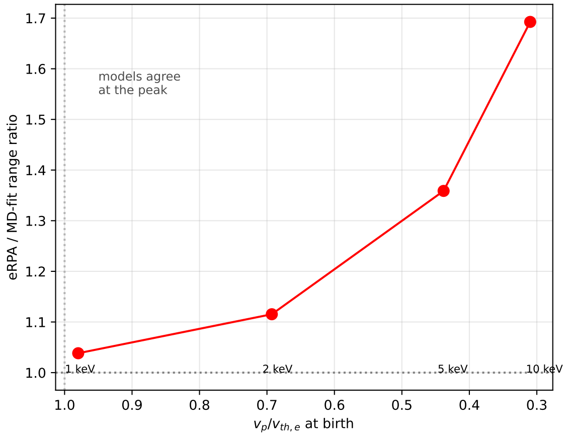
Divergence is purely low-velocity
