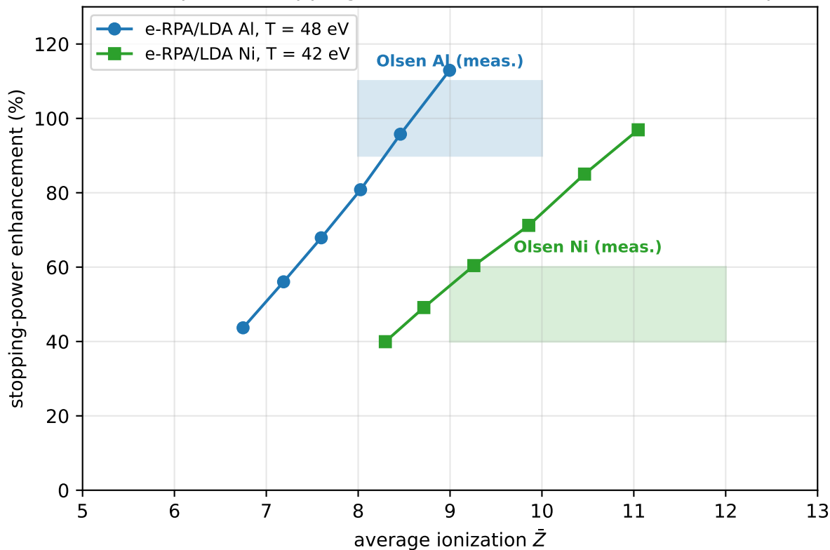
Olsen 1985: proton stopping enhancement at the measured temperatur
