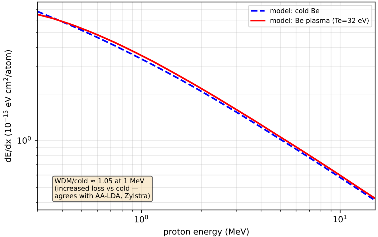
Zylstra 2015: proton in warm dense Be
