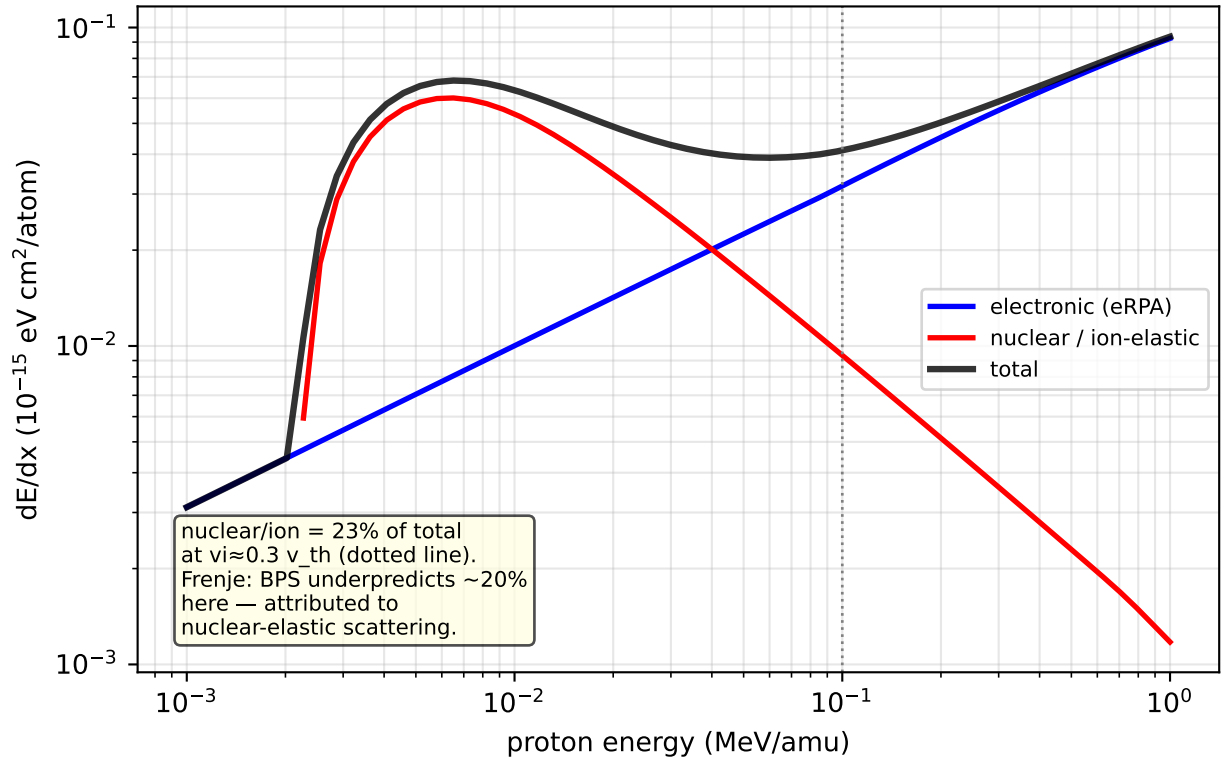
Frenje 2019: ion stopping in DT plasma (Te=2 keV)
