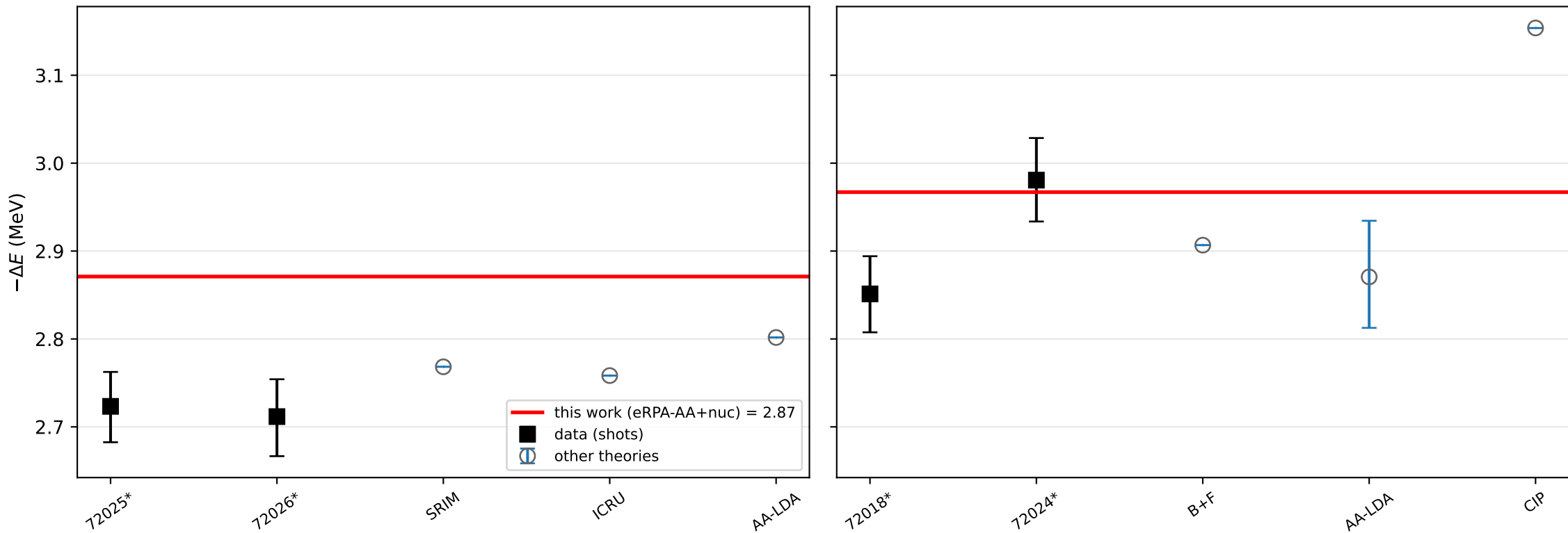
Warm Be (Te \approx 32 eV)
