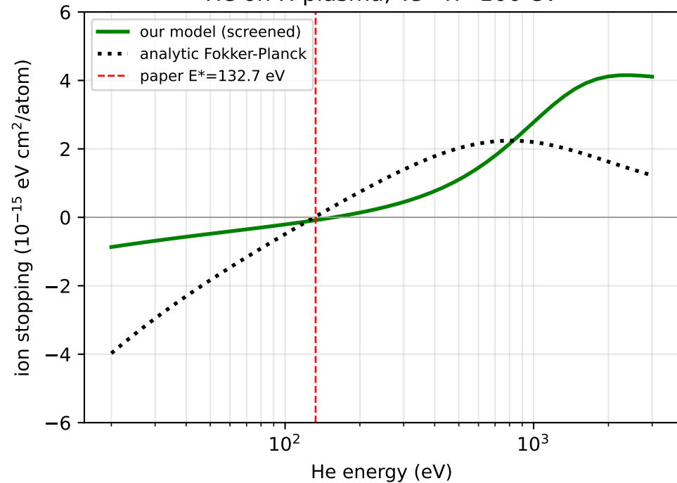
He on H plasma, T_e=T_i=100 eV
