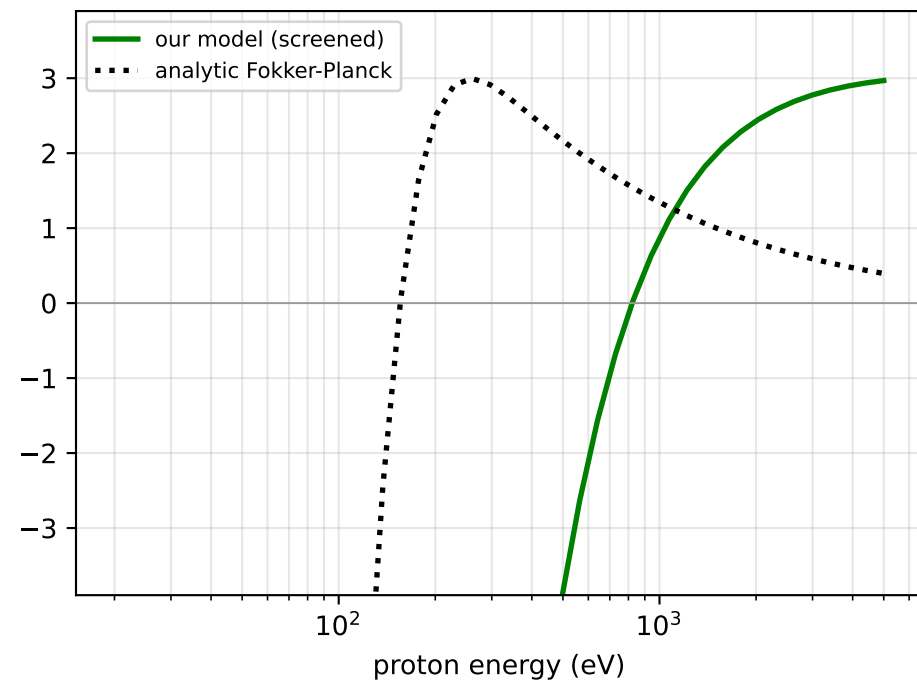
p on Al, T_e=T_i=1000 eV ( \bar{Z}=12.8 )
