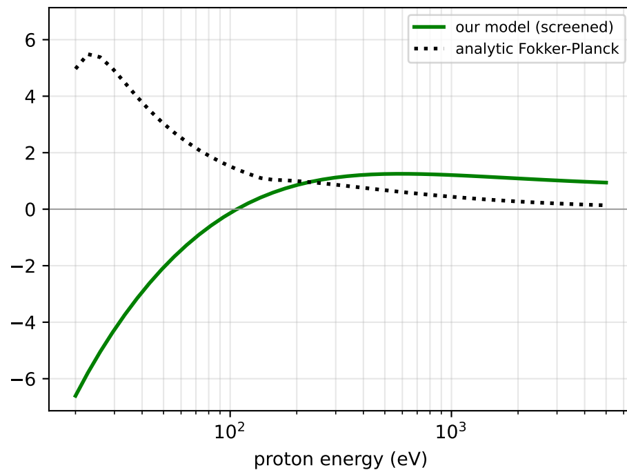
p on Al, T_e=T_i=100 eV ( \bar{Z}=7.9 )
