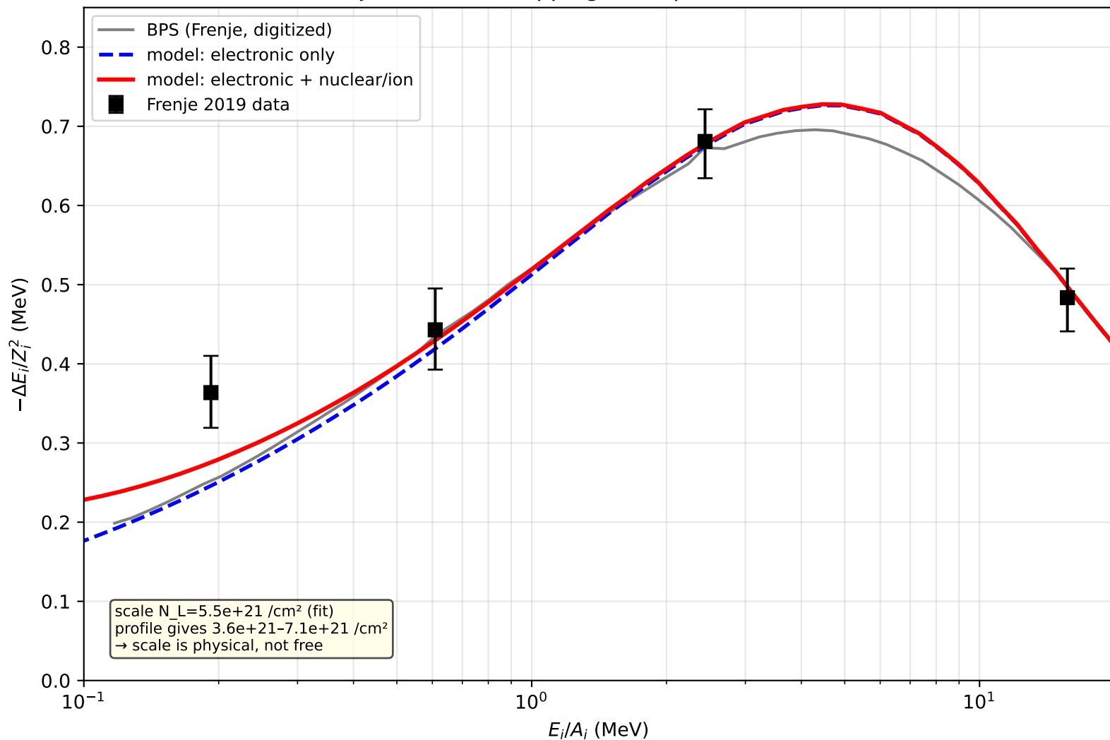
Frenje 2019: ion stopping in DT plasma ( T_e \approx 2 keV)
