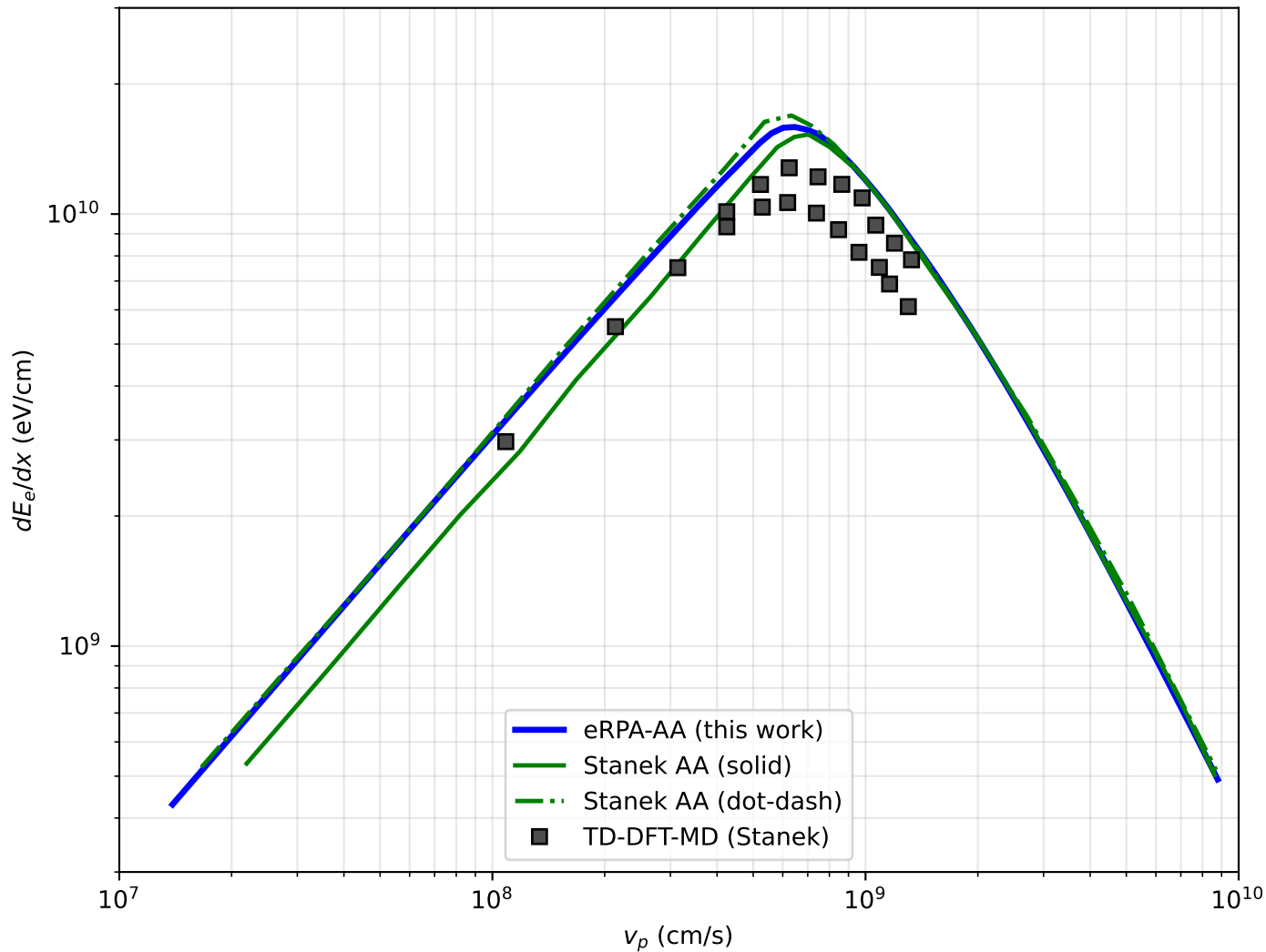
Stanek Fig 12 (b): C, 10 g/cc, 2 eV
