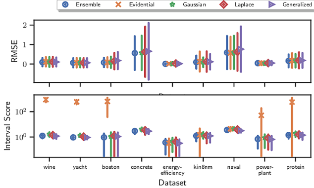
Fig. 4. Benchmark Regression Tasks : RMSE and Interval Score box plot for comparison. The RMSE for all the methods are comparable and lie in same region. In Interval score plot we can see that some methods the score degrades even though their RMSE score is good.
