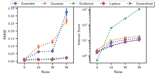
Fig. 3. Breakaway Point estimation: The change in RMSE and Interval Score with respect to outlier percentage in the data for 1D regression dataset. In the first row with clean data all the methods estimate the underlying data and the uncertainty accurately. With increasing outliers the uncertainty estimates are not correct. We observe that the Generalized NLL loss function has the least change in Interval Score with 50% outliers.
