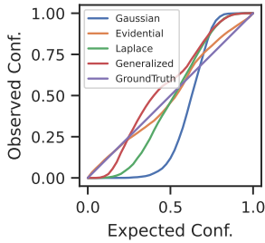
Fig. 6. Uncertainty calibration error: Observed confidence as function of Expected Confidence. For images with adversarial attack the error increases also the uncertainty increases.
