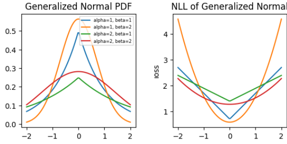
Fig. 2. Probability density function (PDF) (left) and negative log likelihood (NLL) (right) of Generalized normal distribution
