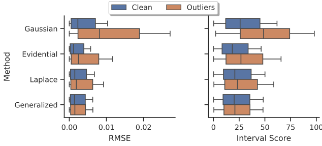
Fig. 5. Clean vs Outliers: RMSE and Interval score comparison for models trained with dataset containing outliers. The difference between both dataset is minimum for generalized loss function.
