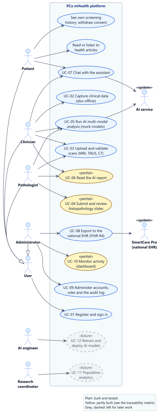
The whole system: use cases UC-01 to UC-12 (research proposal §3.4)
