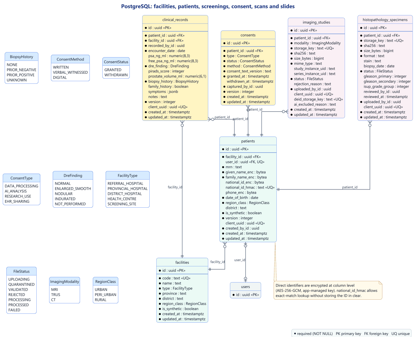
Figure 3.30: ERD: facilities, patients, screenings, consent, scans and slides
