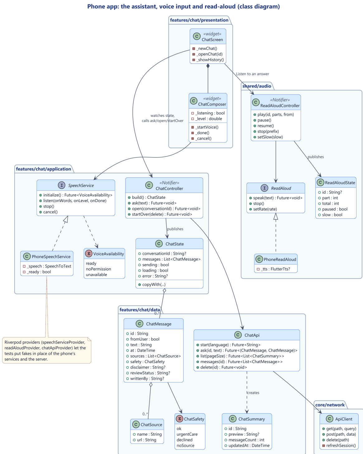
Figure 3.23: Class diagram: the app's assistant, voice input and read-aloud
