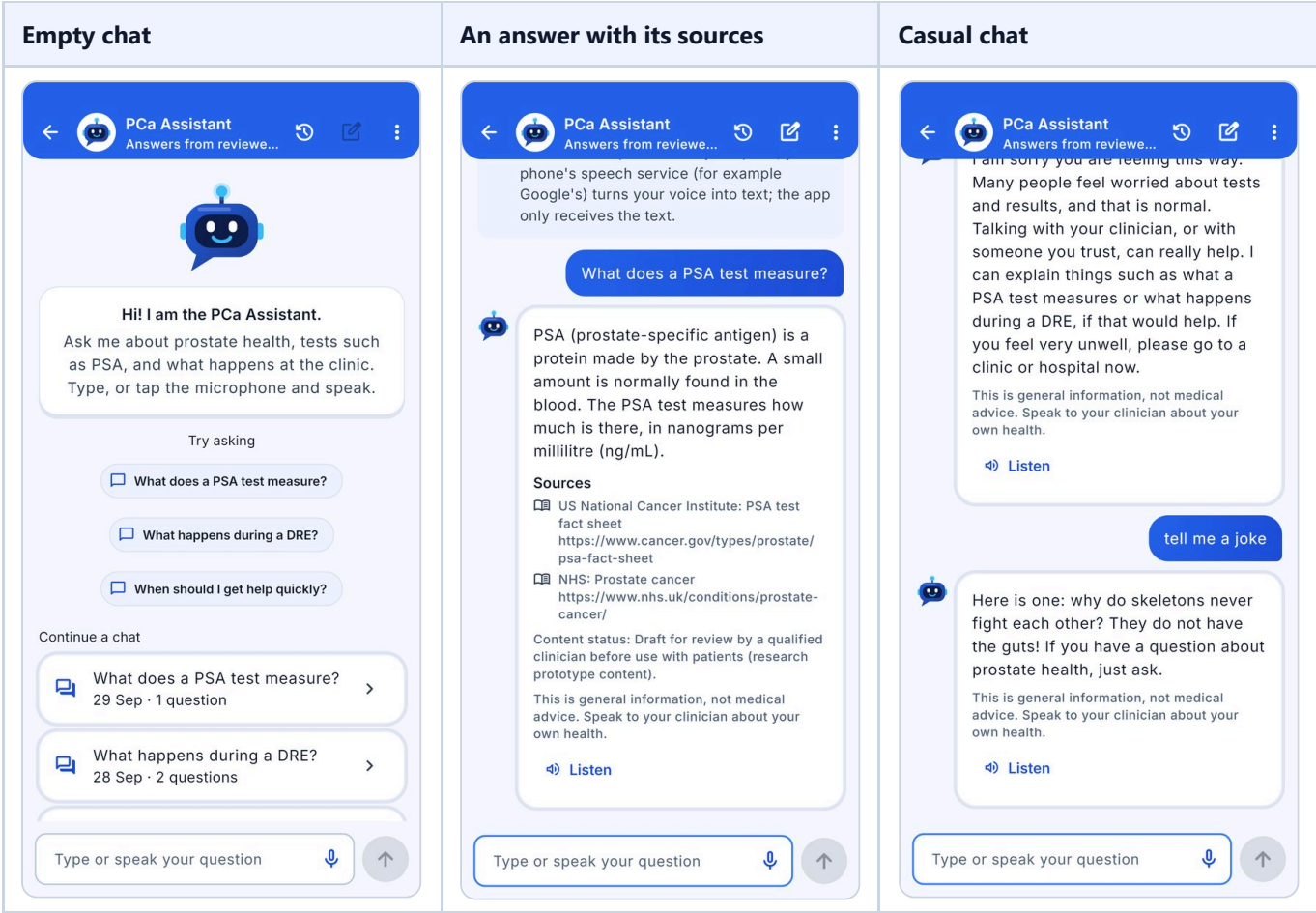
Figure 3.36: Interface design: the assistant
