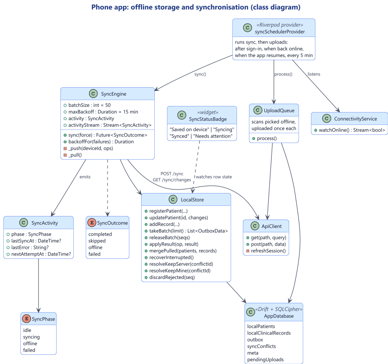
Figure 3.24: Class diagram: the app's offline storage and synchronisation
