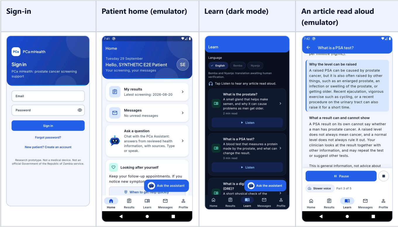
Figure 3.35: Interface design: patient screens
