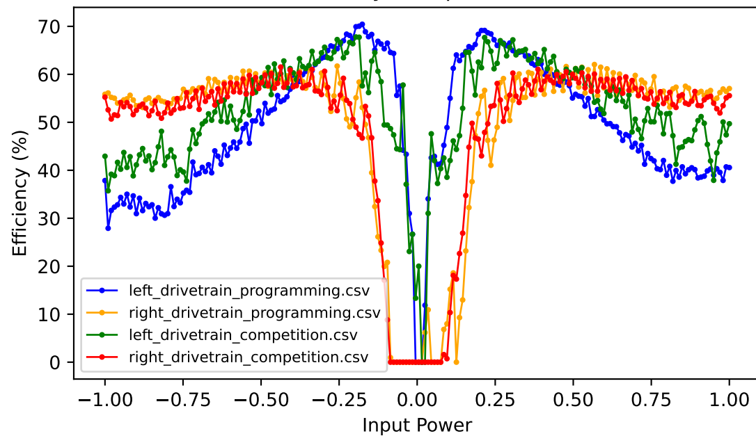
Efficiency vs Input Power
