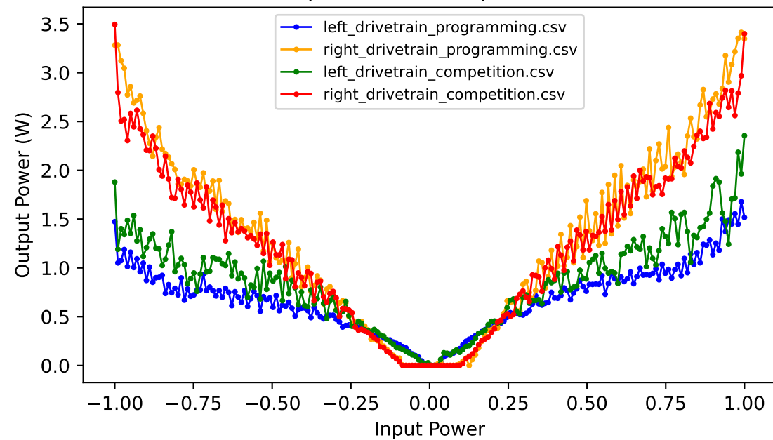
Output Power vs Input Power
