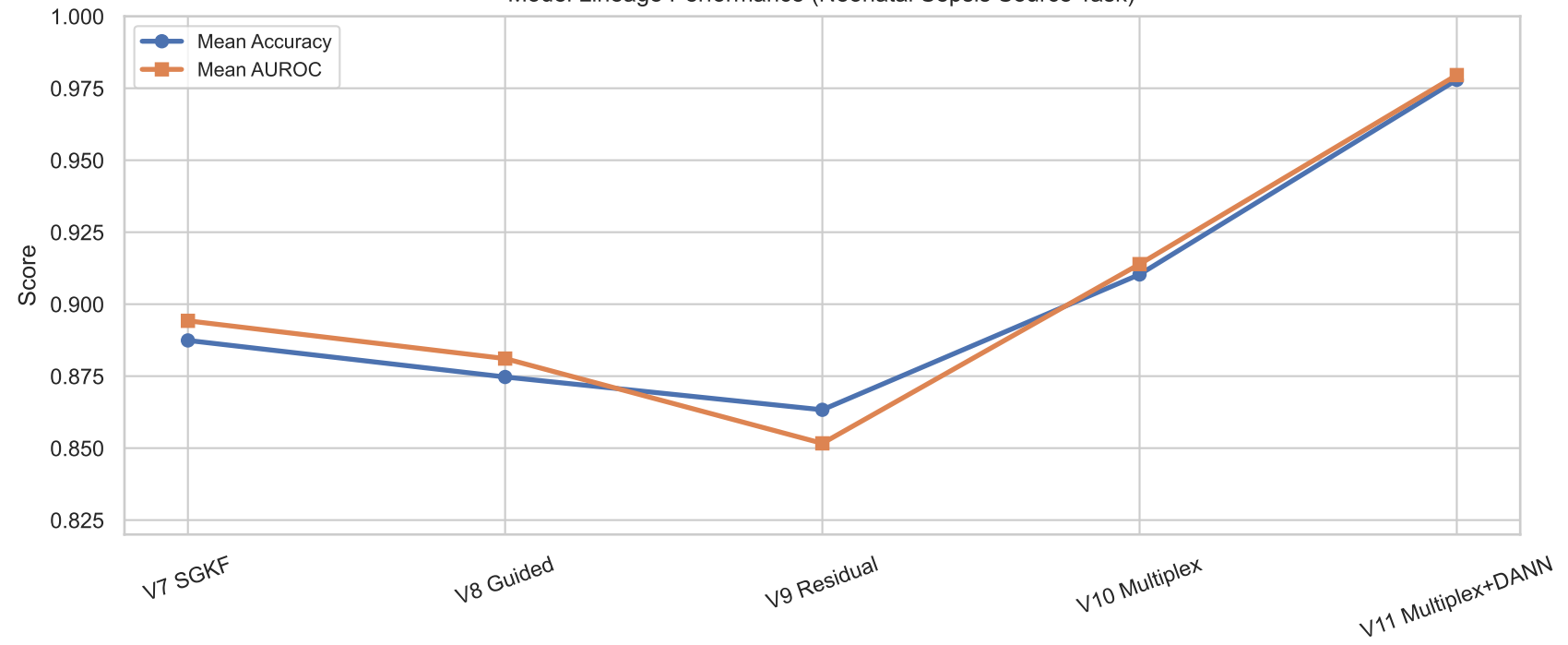
Model Lineage Performance (Neonatal Sepsis Source Task)
