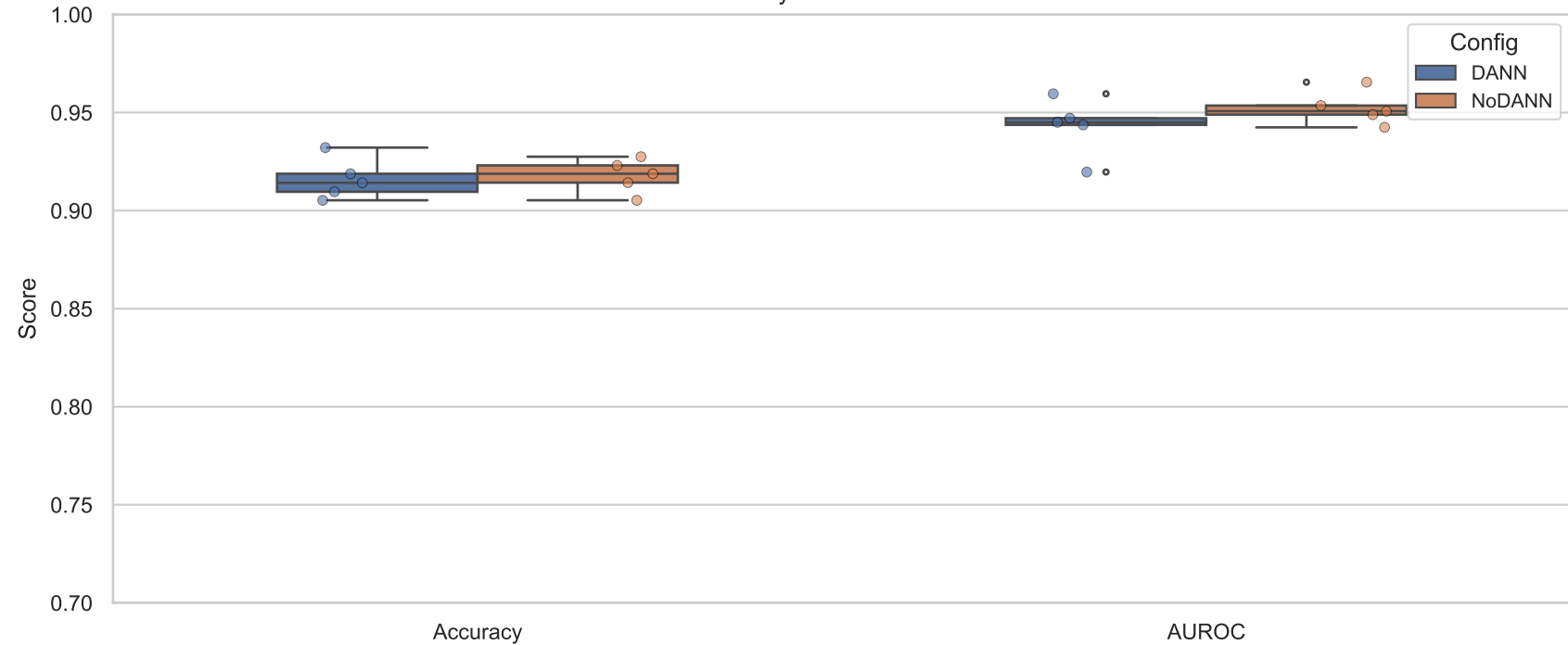
Five-Seed Stability on Brain Alzheimer Transfer
