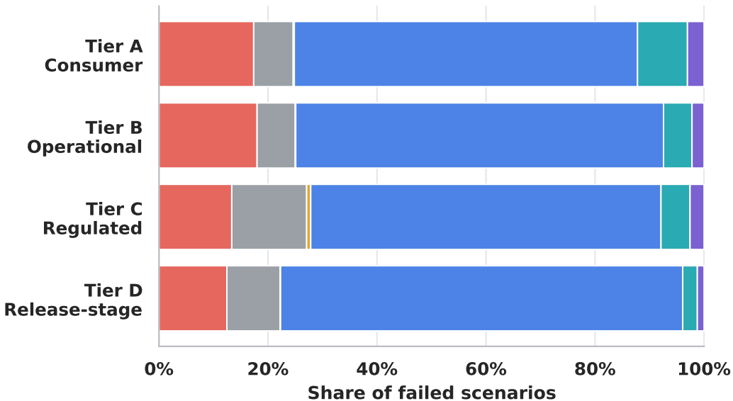
(a) Failure mix by tier
