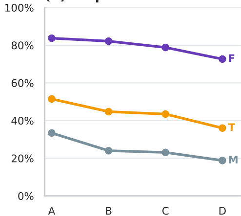
(b) Step-level
