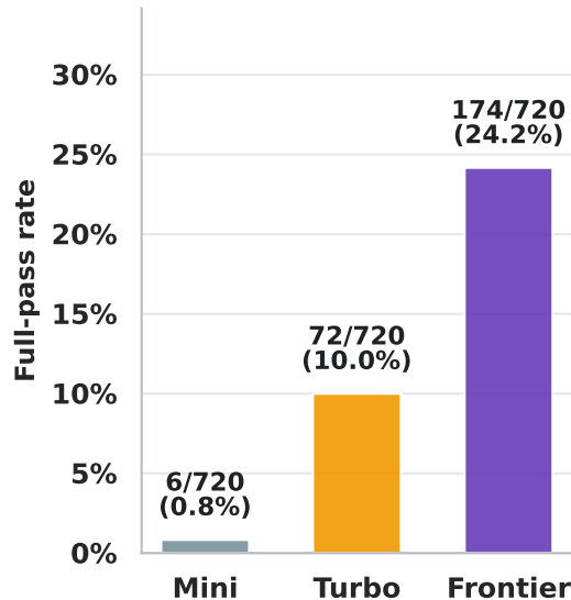
(b) Completion remains hard
