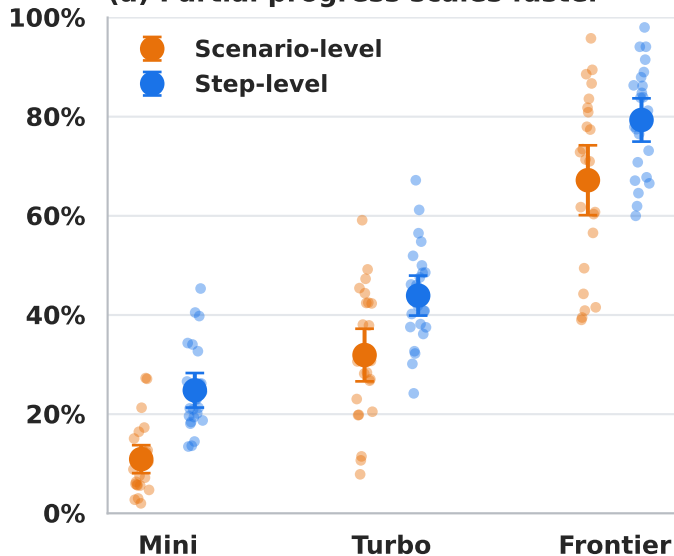
(a) Partial progress scales faster
