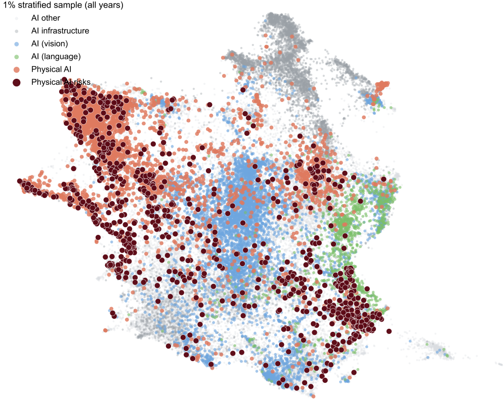
Figure 4. Physical AI document-space diagnostic based on a 1% stratified sample of the integrated AI corpus. Each point is one document, positioned by a two-dimensional projection of its text embedding so that semantically similar documents lie close together; the axes carry no substantive units and are omitted. Colors indicate document groups: AI other (light gray), AI infrastructure (gray), AI vision (blue), AI language (green), and Physical AI (orange). Physical AI risk evidence retained by screening is overlaid as larger dark-red points. The overlay concentrates within and along the edges of the Physical AI regions but also extends into neighboring regions, which is why cross-domain candidates require review of the observed direct harm and approved category boundaries.
