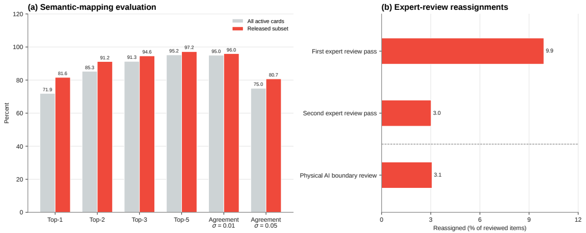
Figure 6. Semantic-mapping evaluation and expert-review outcomes. (a) Top- k category containment and perturbation agreement at two noise scales \sigma for all active cards and the released subset of an earlier taxonomy version. (b) Percentage of reviewed items whose classification was reassigned in two successive expert review passes and in a focused review of Physical AI boundary cases. The reviewed sets differ in scope and selection, so the rates are descriptive only; they should not be compared across reviews or read as measures of accuracy or improvement.
