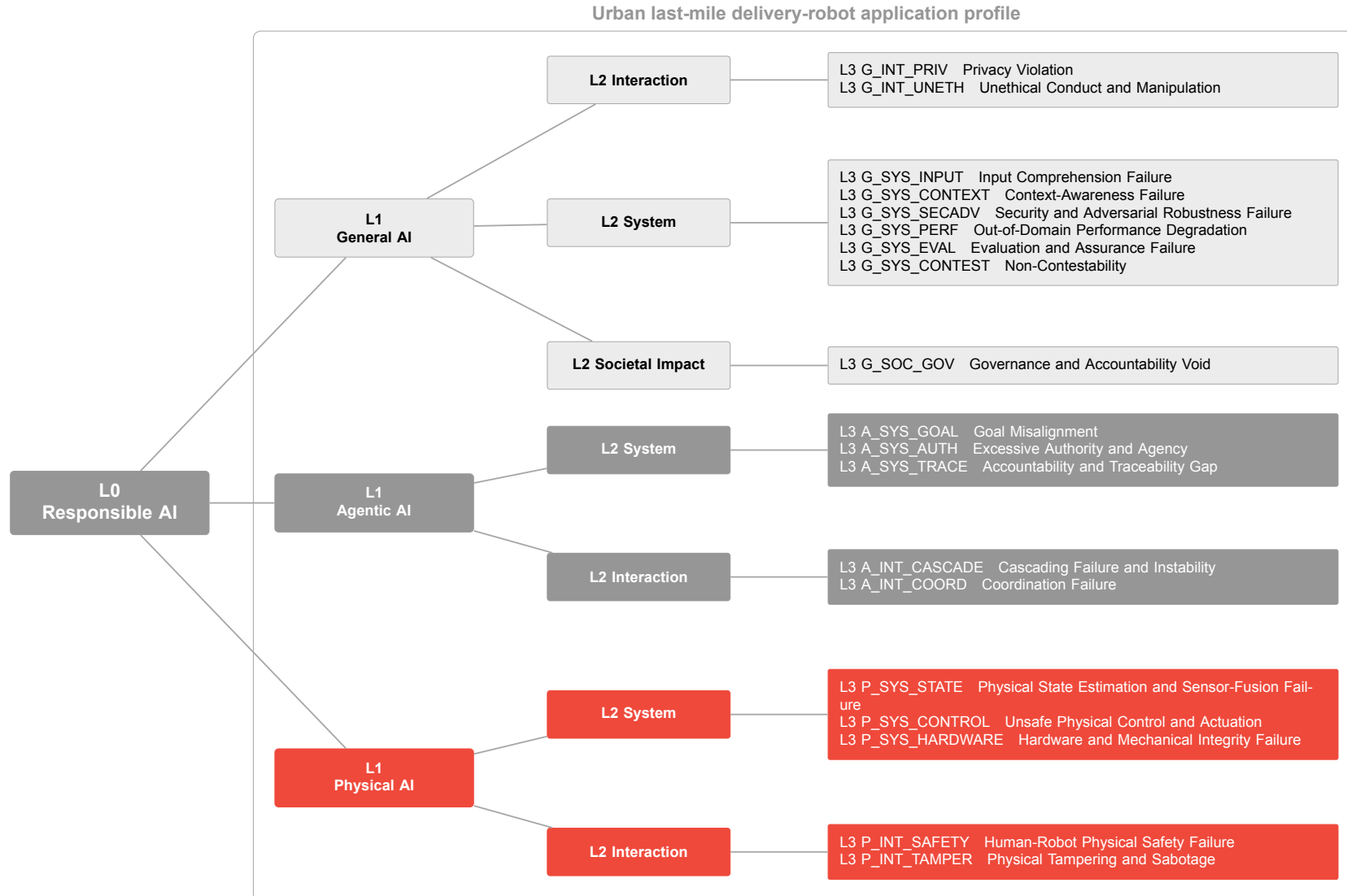
Figure 7. Illustrative service-specific L0–L3 taxonomy for the urban delivery-robot service. The profile selects inherited General AI, Agentic AI, and Physical AI paths while retaining taxonomy IDs and definitions. L4 cards, controls, and evidence are recorded in the service risk register and are not shown in this figure.
