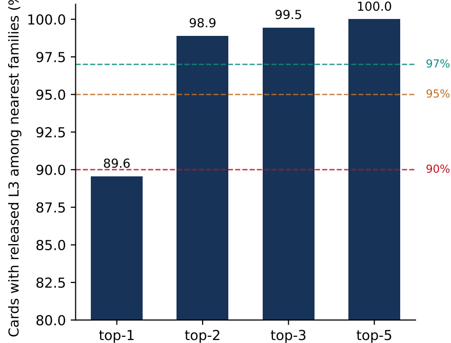
(B) Top-k containment of the released L3
