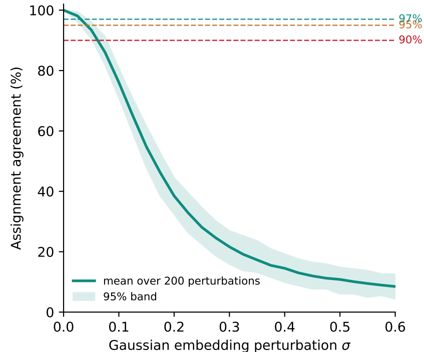
(C) Assignment stability under perturbation
