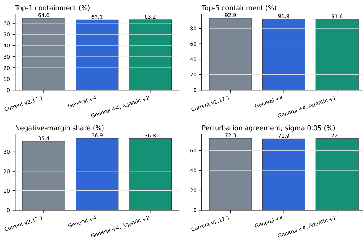
Figure 7: Counterfactual reliability under candidate L3 expansion. Bars compare the current v2.17.1 release with two candidate-expansion conditions. Higher is better for top-1, top-5, and perturbation agreement; lower is better for negative-margin share. Candidate expansion creates plausible movement candidates but does not improve the main reliability criteria.
