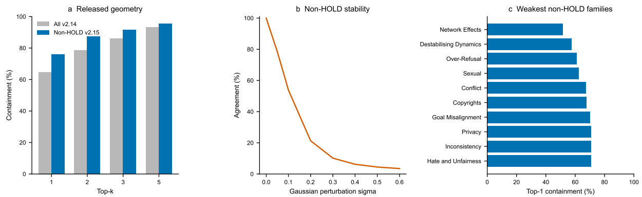
Figure 9: Reliability after HOLD separation (v2.15.0). (a) Top- k containment for the 991 non-HOLD cards is shown against the full v2.14.0 population. (b) Perturbation stability is calculated only on non-HOLD centroids and cards. (c) The ten weakest non-HOLD families identify the next review priorities.
