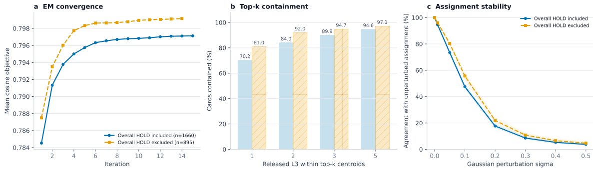
Figure 5: HOLD sensitivity analysis for the full v2.17.2 active release with Physical AI included. (a) Seed-initialized spherical EM reaches a fixed point after 15 iterations with HOLD included and after 14 iterations with HOLD excluded. (b) Released-L3 top- k containment improves across k = 1, 2, 3, 5 after removing HOLD cards from the evaluated active set. (c) Assignment stability under Gaussian embedding perturbation is higher on the non-HOLD subset across the tested noise schedule. Shaded bands indicate 95% intervals across 200 perturbation repeats.
