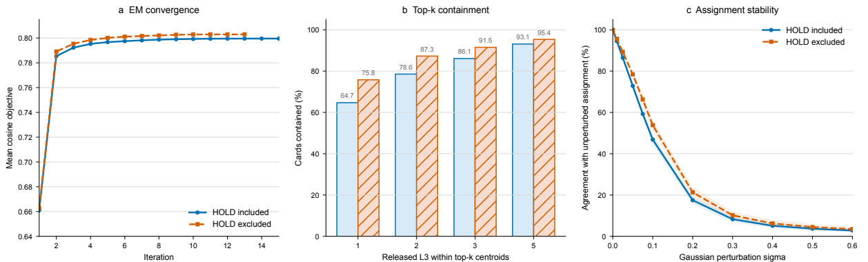
Figure 10: HOLD sensitivity analysis. (a) Seed-initialized spherical EM reaches a fixed point after 15 iterations with HOLD included and after 13 iterations with HOLD excluded. (b) Released-L3 top- k containment improves across k = 1, 2, 3, 5 after removing HOLD cards. (c) Assignment stability under Gaussian embedding perturbation is higher on the non-HOLD subset across the tested noise schedule. Shaded bands indicate 95% intervals across 200 perturbation repeats.
