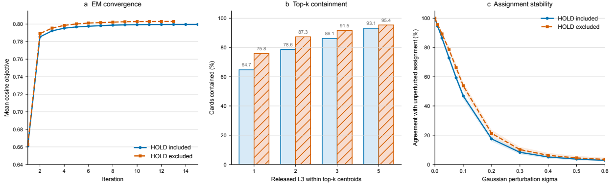
Figure 7: HOLD sensitivity analysis. (a) Seed-initialized spherical EM reaches a fixed point after 15 iterations with HOLD included and after 13 iterations with HOLD excluded. (b) Released-L3 top- k containment improves across k = 1, 2, 3, 5 after removing HOLD cards. (c) Assignment stability under Gaussian embedding perturbation is higher on the non-HOLD subset across the tested noise schedule. Shaded bands indicate 95% intervals across 200 perturbation repeats.
