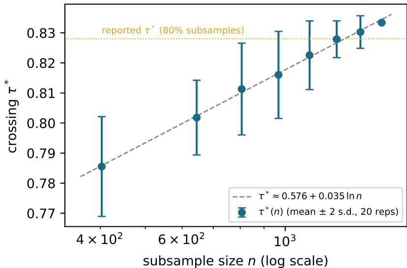
Cohesion-attraction crossing \tau^* increases with inventory size
