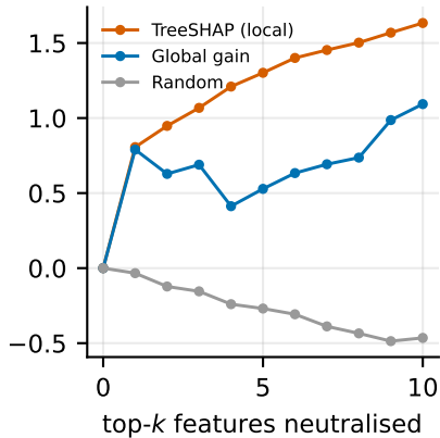
Deletion fidelity: DV
