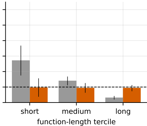
BV random
