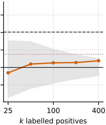
BV project
