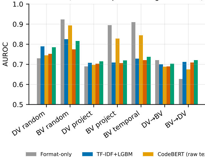
Detection (raw text exploits the Big-Vul artifact)
