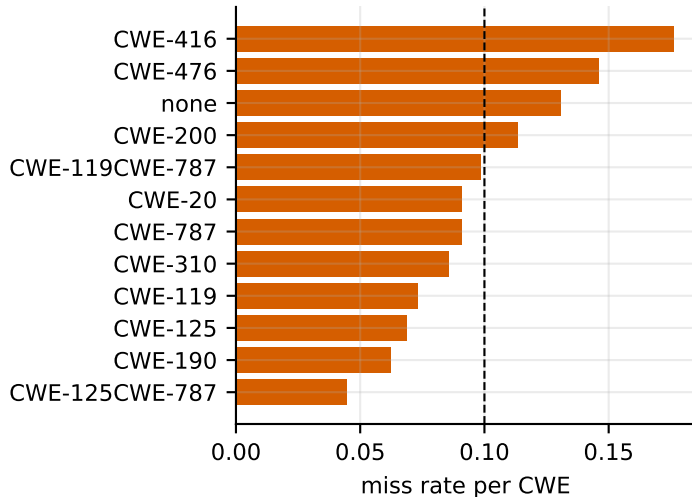
DV random (LightGBM, \alpha = 0.10 )
