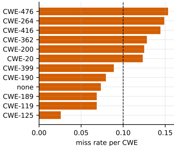
BV random (LightGBM, \alpha = 0.10 )
