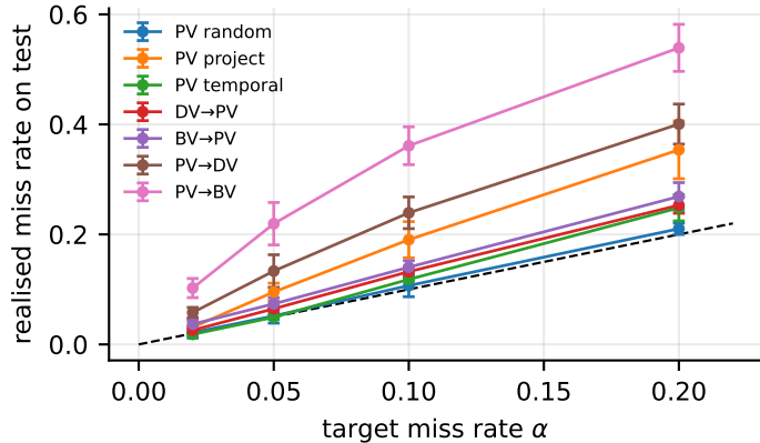
PrimeVul: source-calibrated clearance
