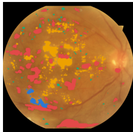
Pixel masks
