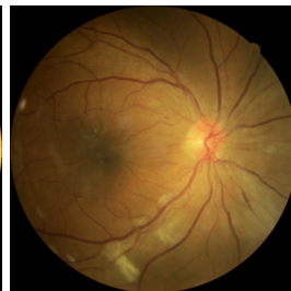
DDR train #295
