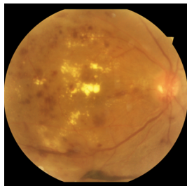
DDR train #366
