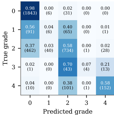
(a) Confusion (row-normalised)
